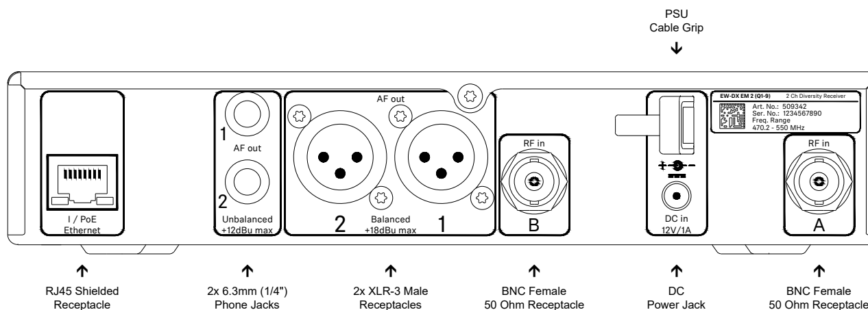
REAR View
