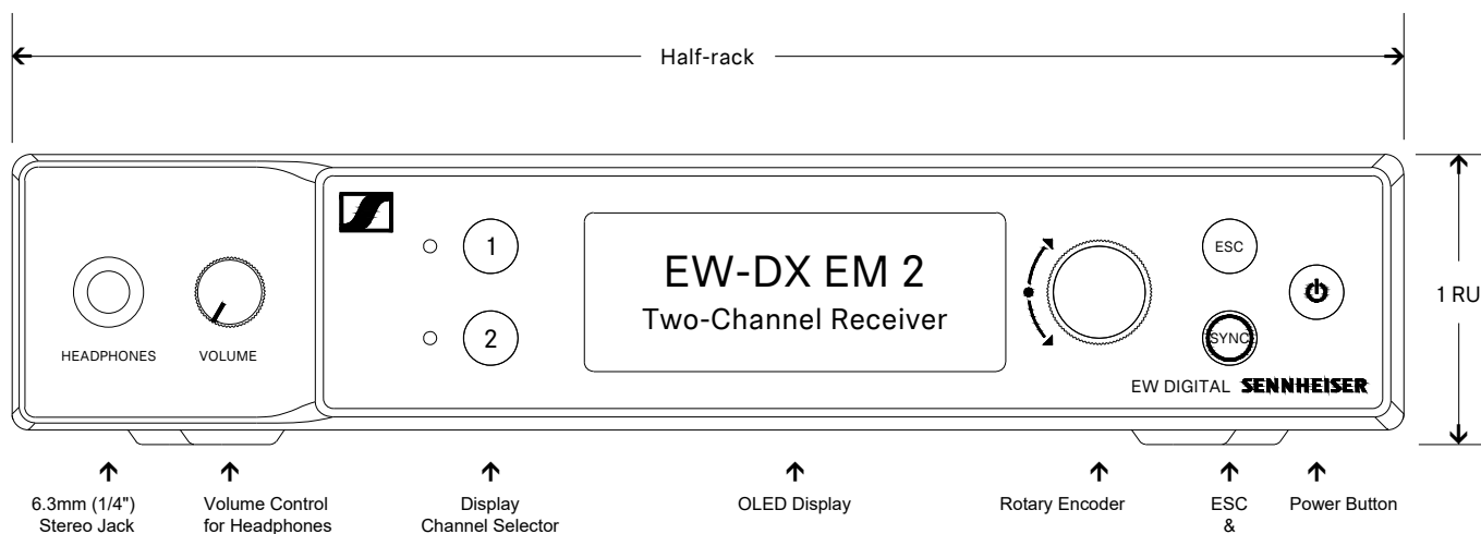
FRONT View
